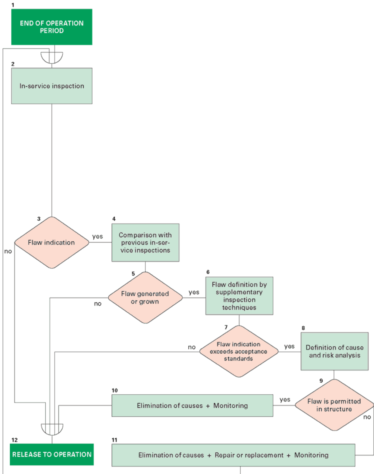
Flow chart for the evaluation of inspection results [29]. [2019-02-15 ]
